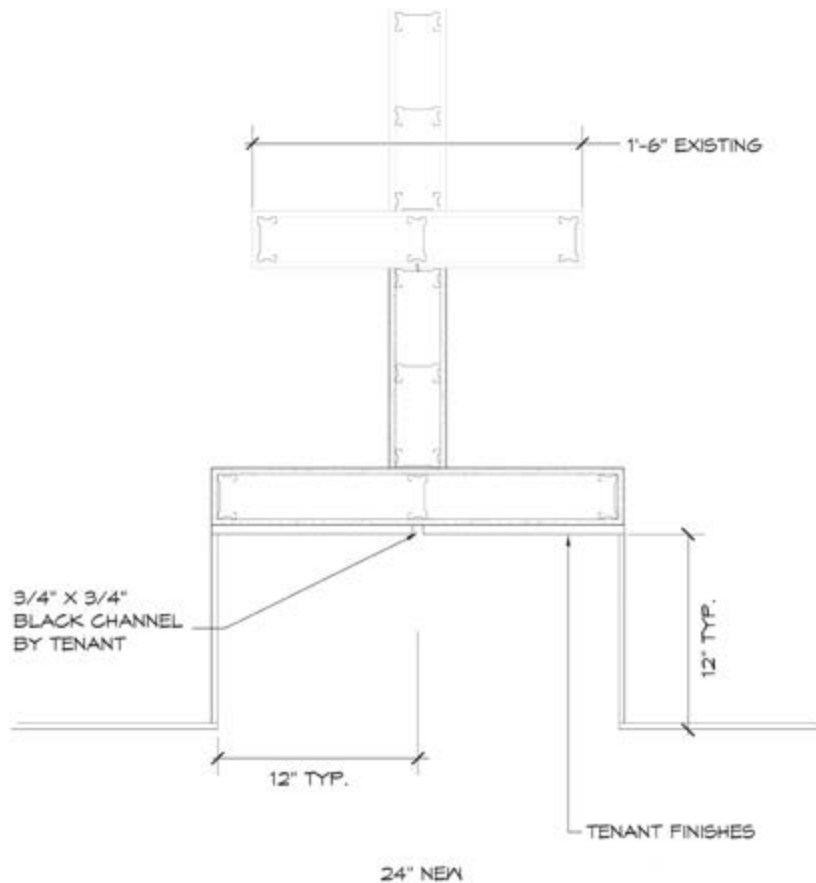
PLAN DETAIL @ NEUTRAL CHANNEL CONDITION SCALE: NTS
